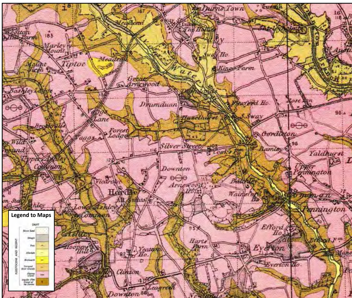
Geological Map in area of Parish
