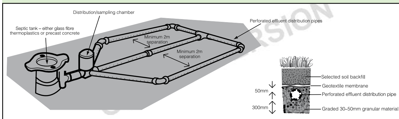
Diagram 1 Drainage field
