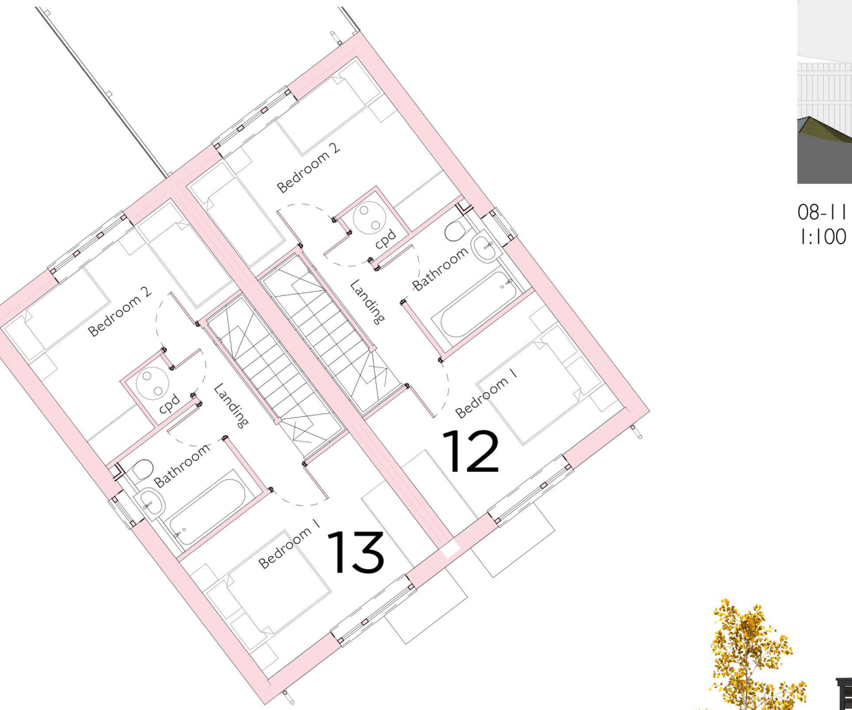
First Floor 1:100
