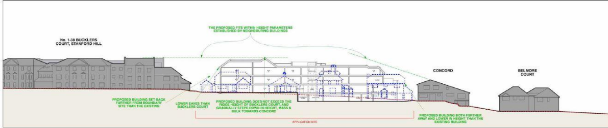
Indicative Site Section - showing design response to existing site topography Not to Scale
